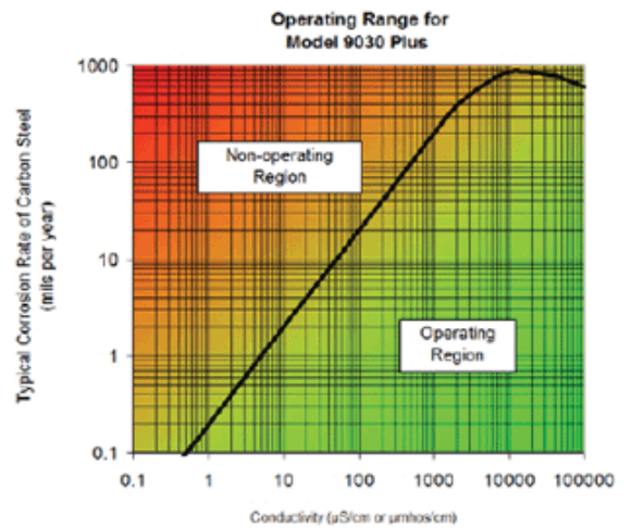
Note: Based on 20% error limit (see ASTM G96)
